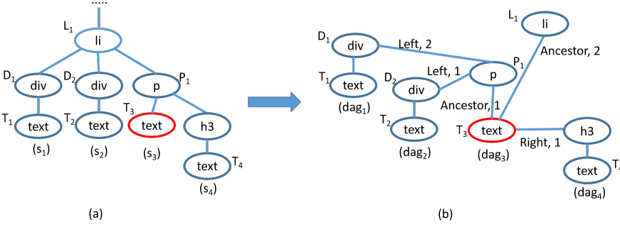
Fig. 17. An example demonstrating the transformation from an HTML document to a predicates graph.
