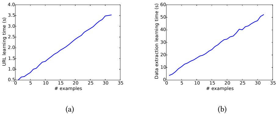
Fig. 24. The synthesis time vs the number of examples for URL learning (a) and data extraction learning (b).
