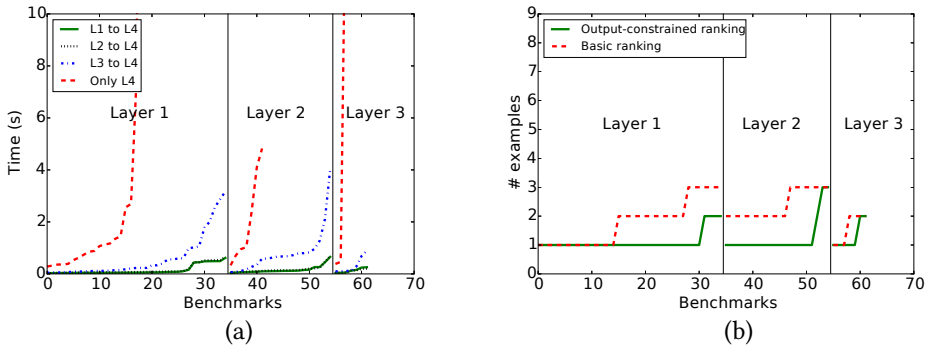
Fig. 22. (a) The synthesis times and (b) the number of examples required for learning URL programs. The benchmarks are categorized based on the layer that contains the program required for performing the transformation.
