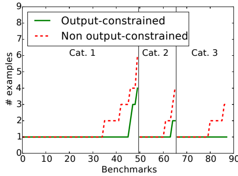
Fig. 25. The number of examples needed to learn the data extraction programs.
