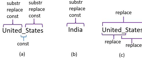
Fig. 12. (a) and (b) shows a portion of the DAGs for Ex 4.3 using layer 1 of hierarchical search. (c) shows additional edges from layer 2 of the hierarchical search.
