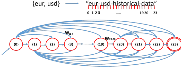
Fig. 8. An example DAG using Version space algebra (VSA) to represent the set of transformations consistent with the example. For example, here, \mathcal{W}_{0,3} is a list of three different expressions \{\text{ConstStr}(\text{eur}), \text{SubStr}(0, \text{ConstPos}(0), \text{ConstPos}(-1), \text{lower}), \text{AnyStr}\} ; \mathcal{W}_{19,20} = \{\text{ConstStr}(d), \text{SubStr}(1, \text{ConstPos}(2), \text{ConstPos}(3), \text{lower}), \text{AnyStr}\} .
