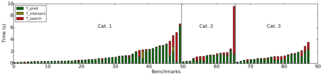
Fig. 23. The synthesis times for learning data extraction programs by WEBRELATE on the 88 benchmarks.
