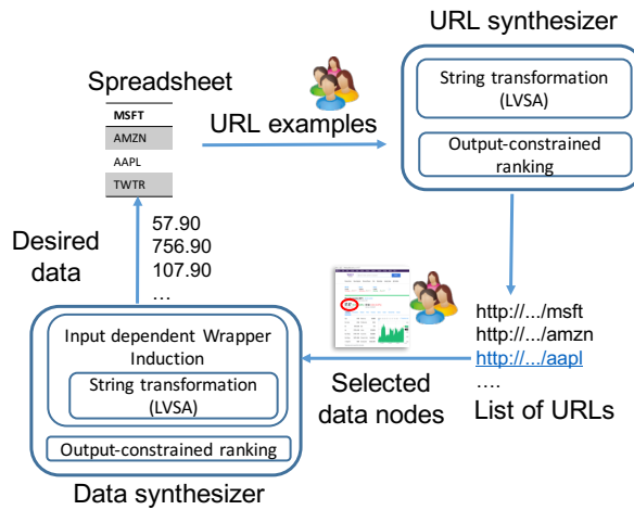
Fig. 2. An overview of the workflow of the WEBRELATE system. A user starts with providing a few examples for URL strings corresponding to the desired webpages of the first few spreadsheet rows. The URL synthesizer then learns a program consistent with the URL examples, which is executed to generate the desired URLs for the remaining spreadsheet rows. The user then opens the URLs for the first few spreadsheet rows in an adjoining pane (one at a time), and highlights the data items that need to be extracted from the webpage. The Data synthesizer then learns a data extraction program consistent with the examples to extract the desired data for the remaining spreadsheet rows.
